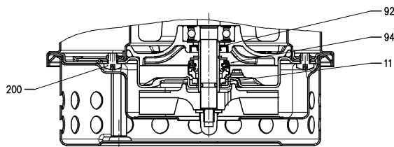
MOTOR FIXING
