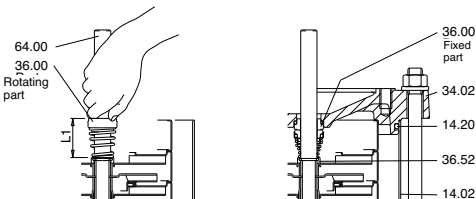
Fig.4 Inserting the mechanical seal
