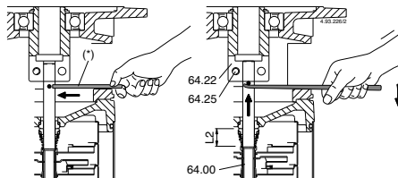
Fig. 5a Rotor rested, with shaft not locked in the coupling.
