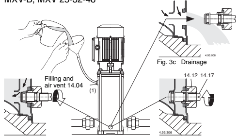
Fig. 3a Filling: internal passage open
